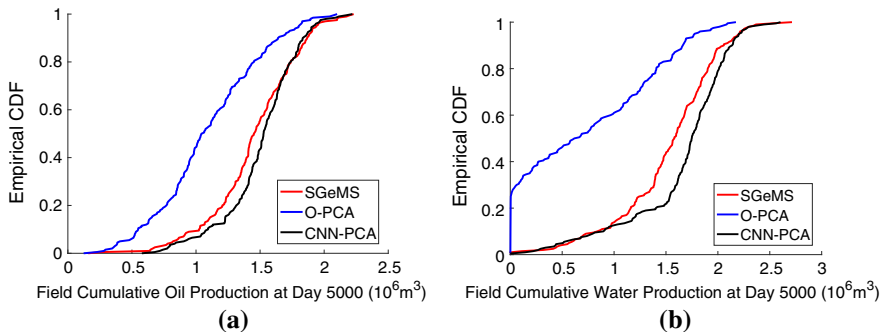
Fig. 17 Statistics of cumulative field oil and water production at the end of the simulation from (new) SGeMS models, O-PCA models, and CNN-PCA models. a Cumulative oil production CDFs and b cumulative water production CDFs
